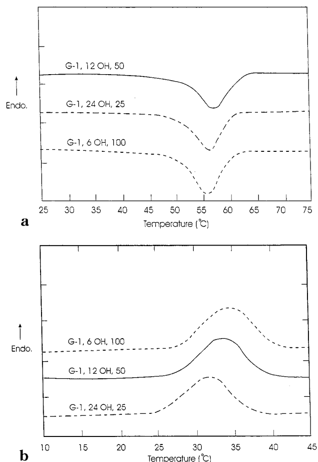
Figure 10. (a) DSC thermograms of dendrimer-like star polymers organized in Scheme 2 along the line denoted as G-1 (a) melting region and (b) crystallization region. (b) DSC thermograms of dendrimer-like star polymers organized in Scheme 2 along the line denoted as G-1 (a) melting region and (b) crystallization region.
