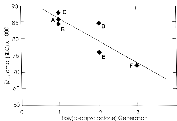
Figure 5. Number-average molecular weight M_n versus the different generations of poly( \epsilon -caprolactone) in the dendrimer-like star polymers; (A) G-1, 6 OH 100 , (B) G-1 12 OH, 50 , (C) G-1, 24 OH, 25 , (D) G-2, 6 OH, 33.3 , (E) G-2 12 OH 16.7 , (F) G-3, 6 OH 14.3 .
